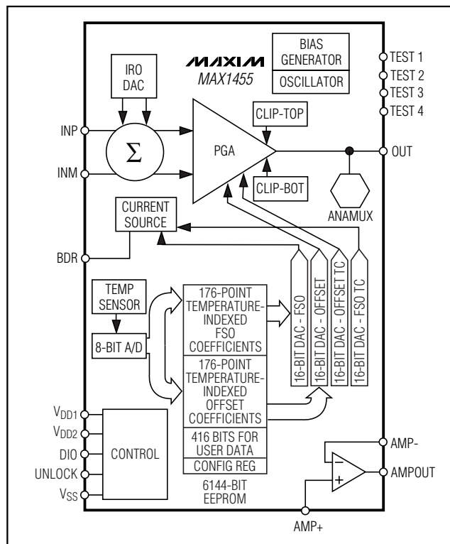
Figure 1. Functional Diagram
