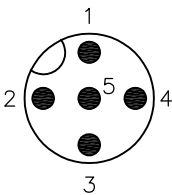
Contact Layout Male
