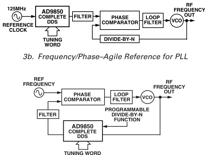
3c. Digitally-Programmable Divide-by-N Function in PLL
