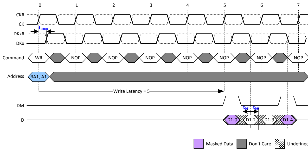
Basic WRITE Burst with DM Timing: BL=4 & WL=5
