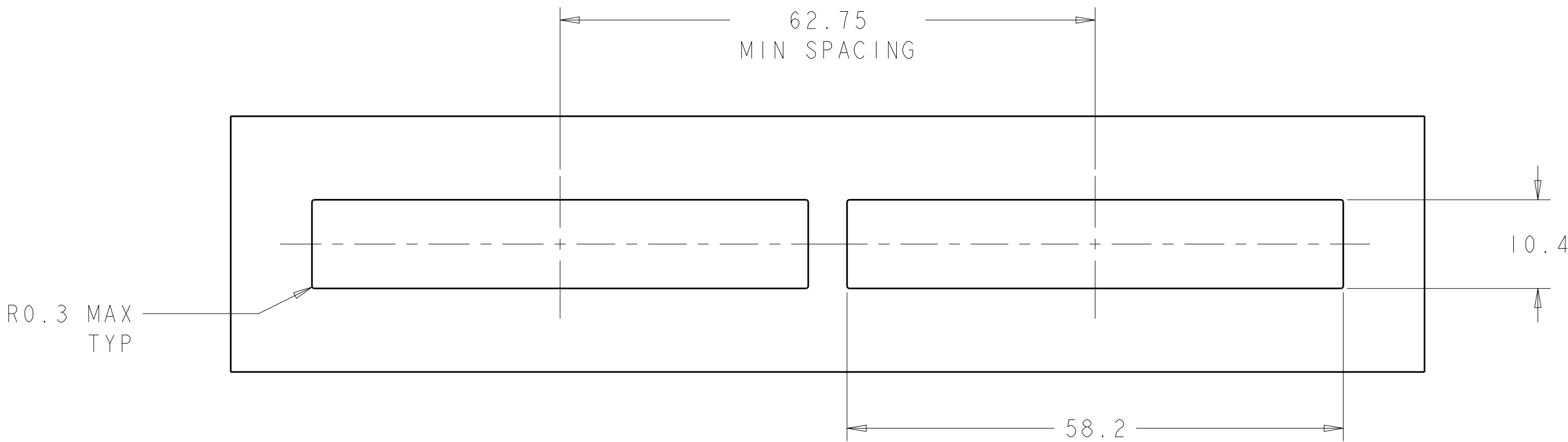
RECOMMENDED BEZEL CUT-OUT SINGLE SIDED APPLICATIONS SCALE 2:1
