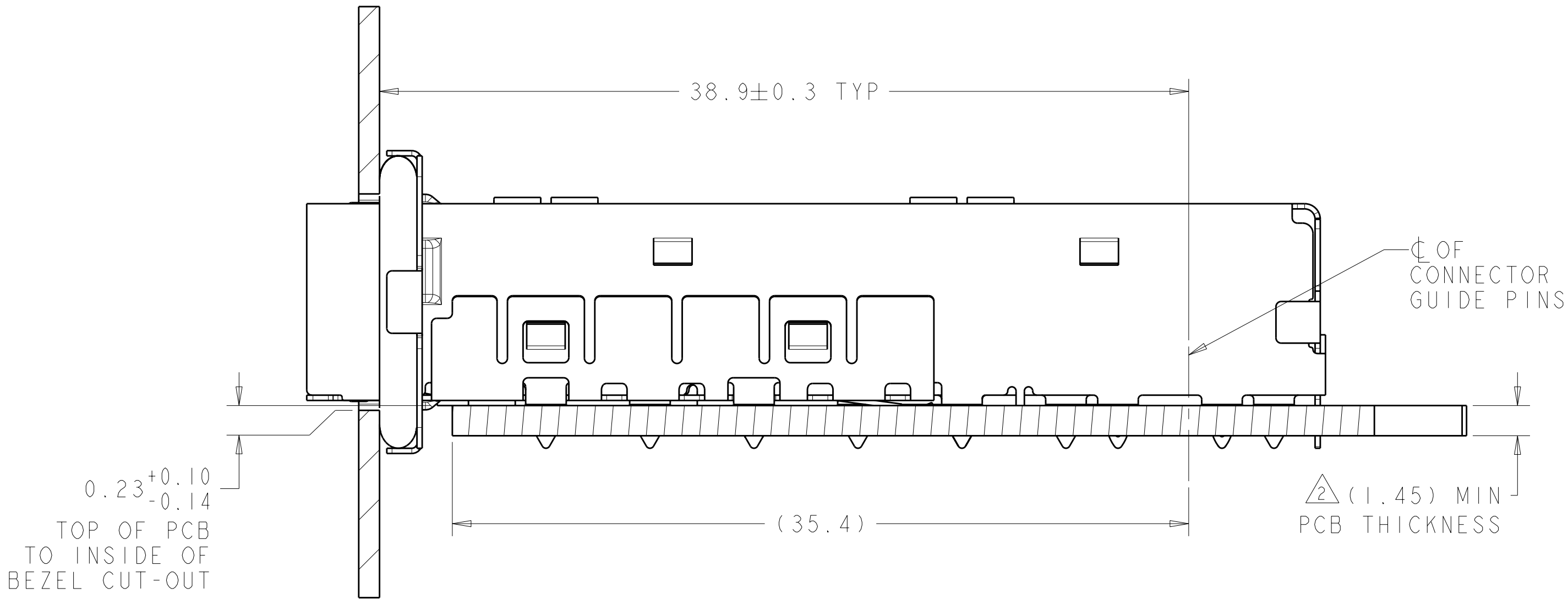
2057353-1 MOUNTED ON PC BOARD SHOWN THRU RECOMMENDED BEZEL SECTION
