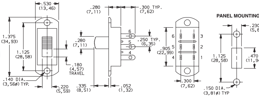
S202031SS03Q DPDT
