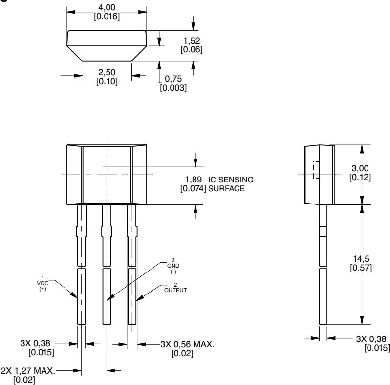
Figure 6. SM451R and SM453R Mounting Dimensions (For reference only. mm/[in].)
