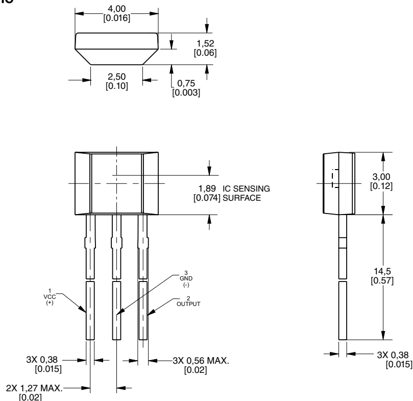
Figure 6. SM451R and SM453R Mounting Dimensions (For reference only. mm/[in].)
