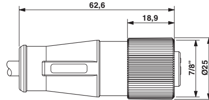
Dimensioned drawing
