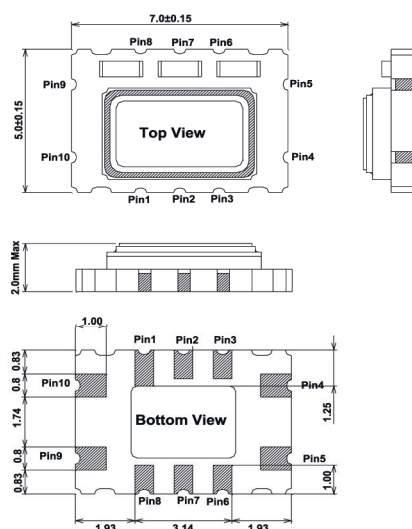
Pin Connection
