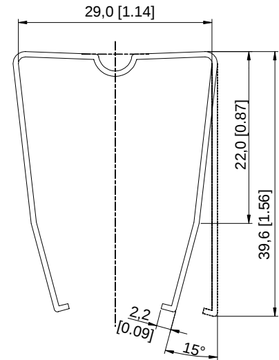
Figure 2. Dimensions
