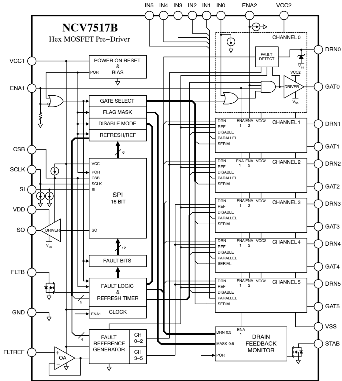
Figure 1. Block Diagram
