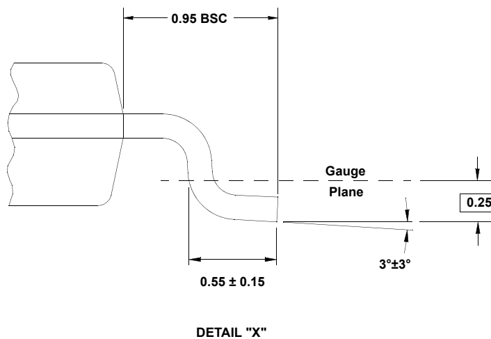
DETAIL "X"
