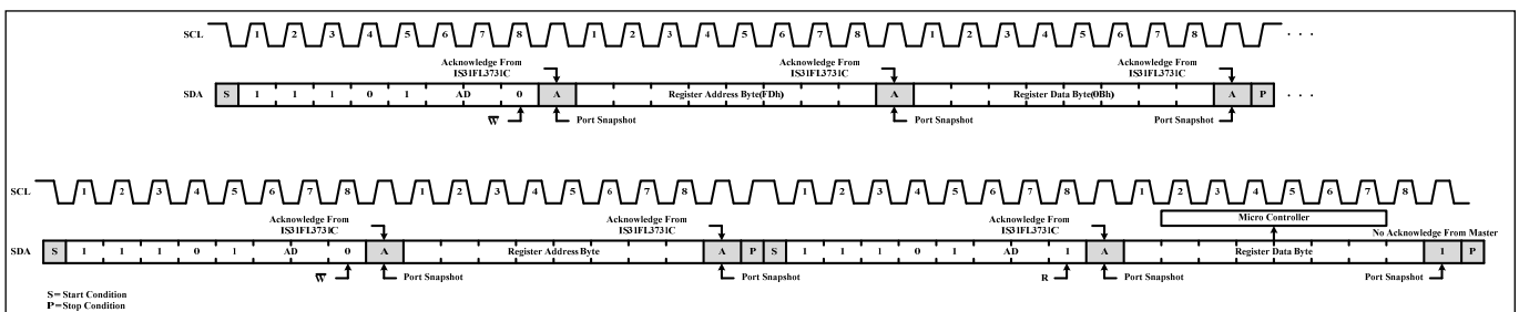
Figure 7 Reading from IS31FL3731C
