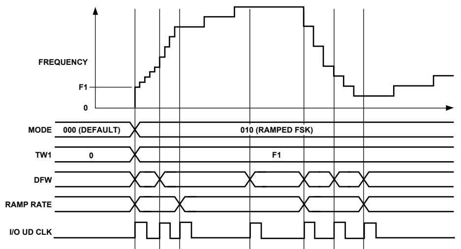
Figure 41. Example of a Nonlinear Chirp
