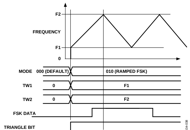
Figure 38. Automatic Linear Ramping Using the Triangle Bit
