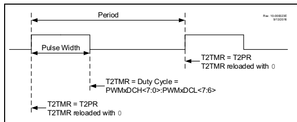
FIGURE 24-2: PWM OUTPUT
