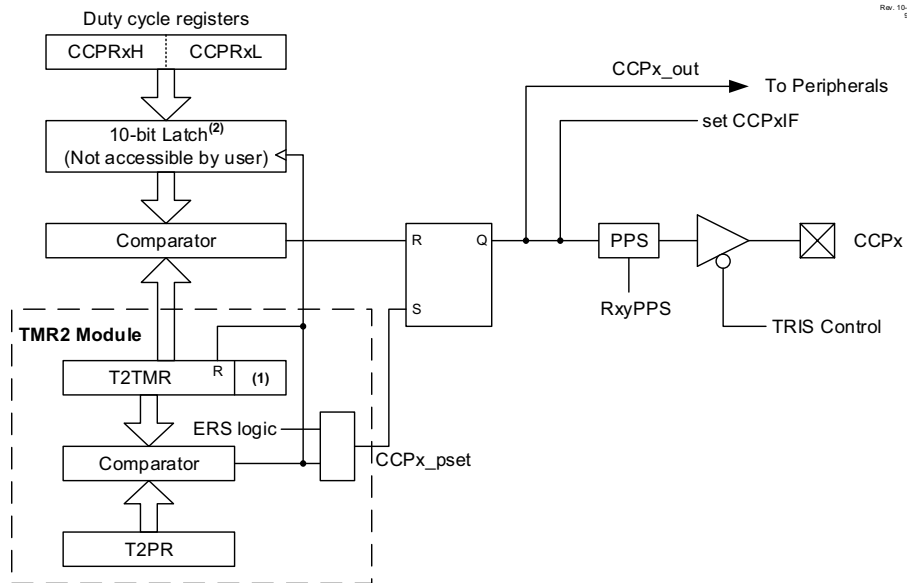
FIGURE 23-4: SIMPLIFIED PWM BLOCK DIAGRAM
