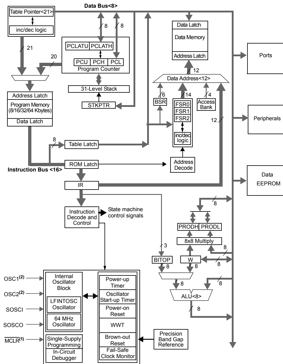
FIGURE 3-1: PIC18(L)F26/27/45/46/47/55/56/57K42 FAMILY BLOCK DIAGRAM
