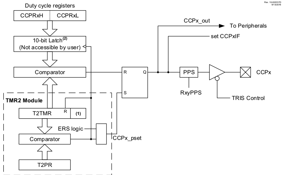
FIGURE 23-4: SIMPLIFIED PWM BLOCK DIAGRAM
