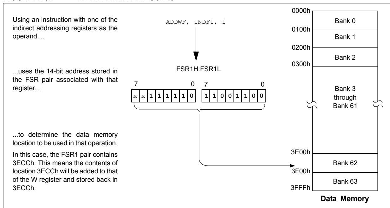
FIGURE 4-6: INDIRECT ADDRESSING
