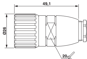
Dimensional drawing
