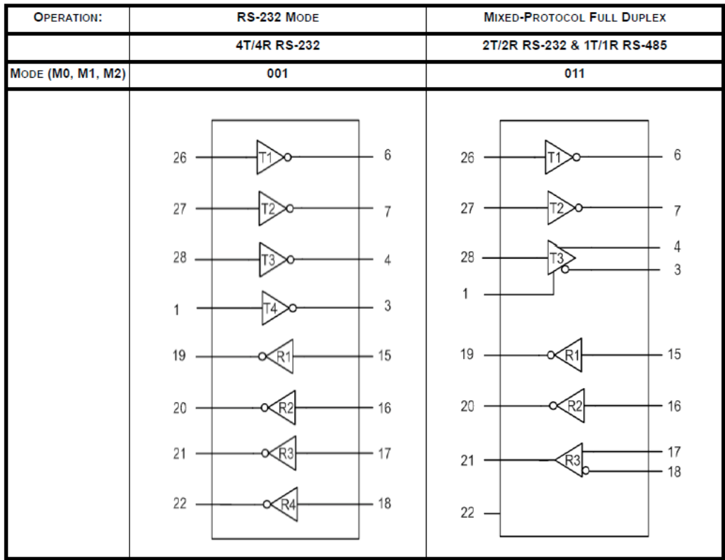
Figure 1- Mode Configuration
