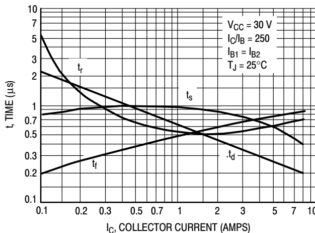
Figure 4. Typical Switching Times
