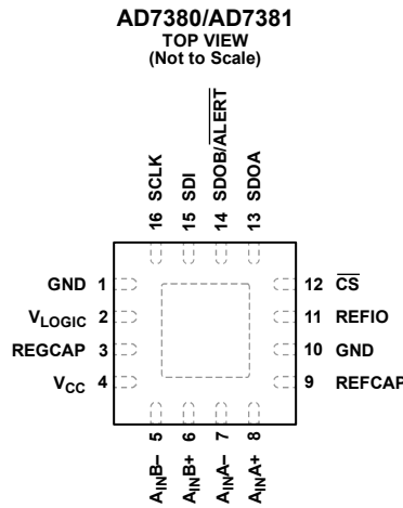
Figure 8. Pin Configuration
