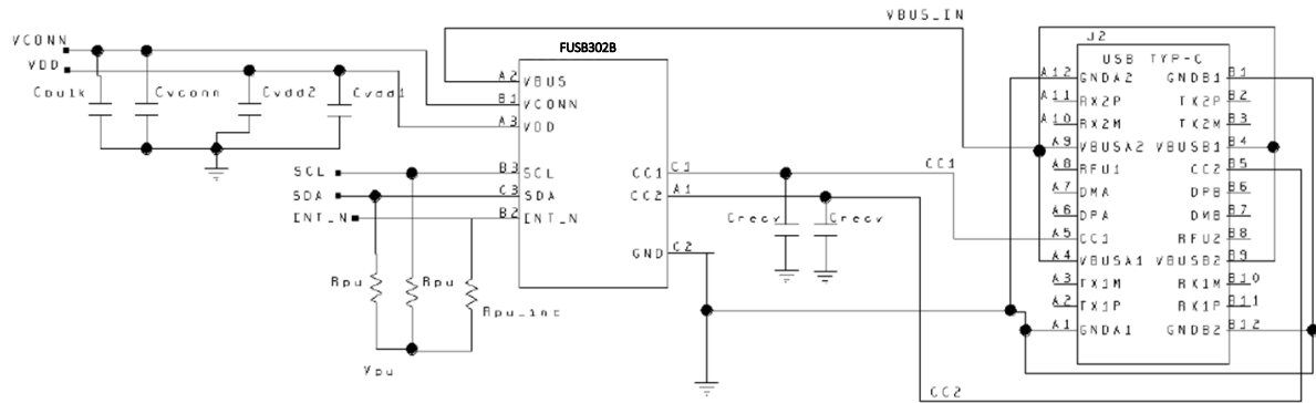
Figure 17. FUSB302/FUSB302B Reference Schematic Diagram
