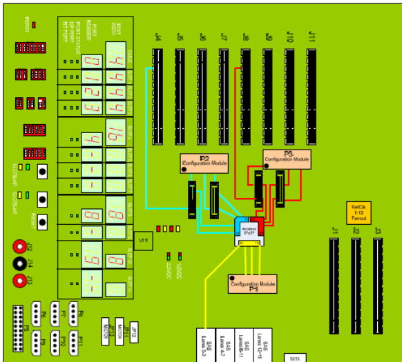
Figure 9. PEX 8724 RDK
