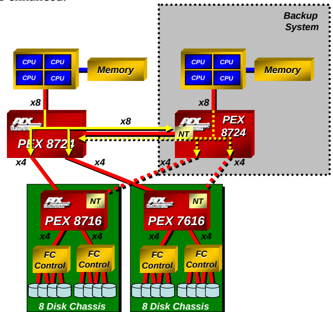
Figure 8. N+1 Failover
