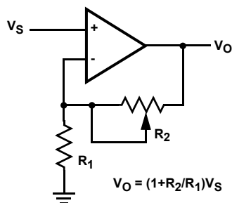
FIGURE 12. NONINVERTING AMPLIFIER
