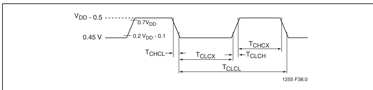
Figure 38: External Clock Drive Waveform
