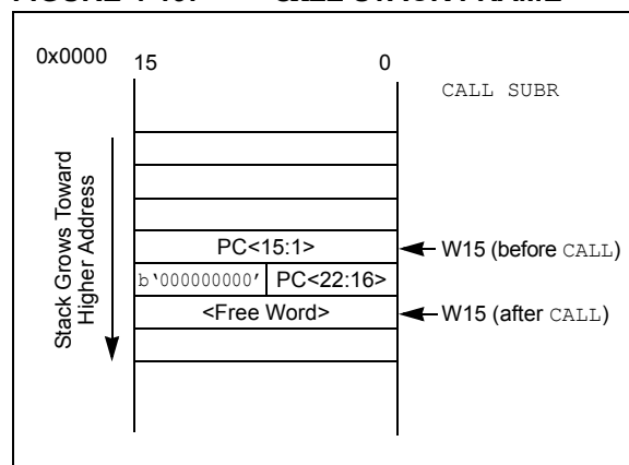
FIGURE 4-19: CALL STACK FRAME
