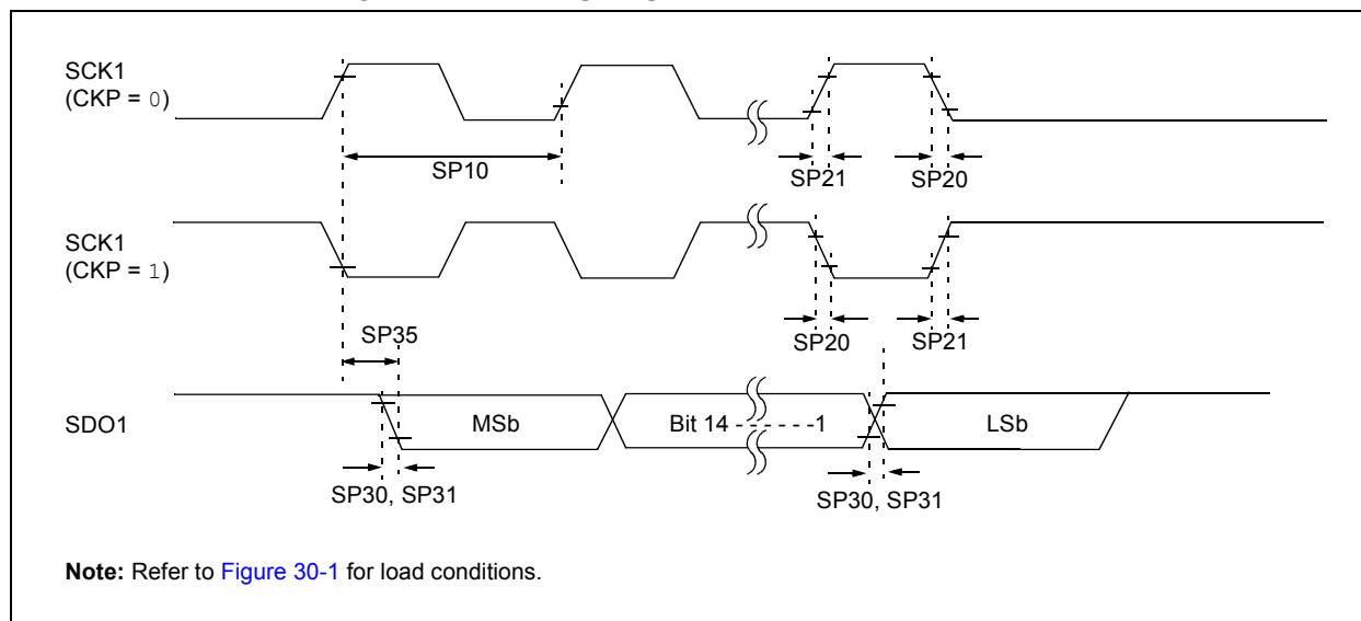
FIGURE 30-22: SPI1 MASTER MODE (HALF-DUPLEX, TRANSMIT ONLY, CKP = 0) TIMING CHARACTERISTICS
