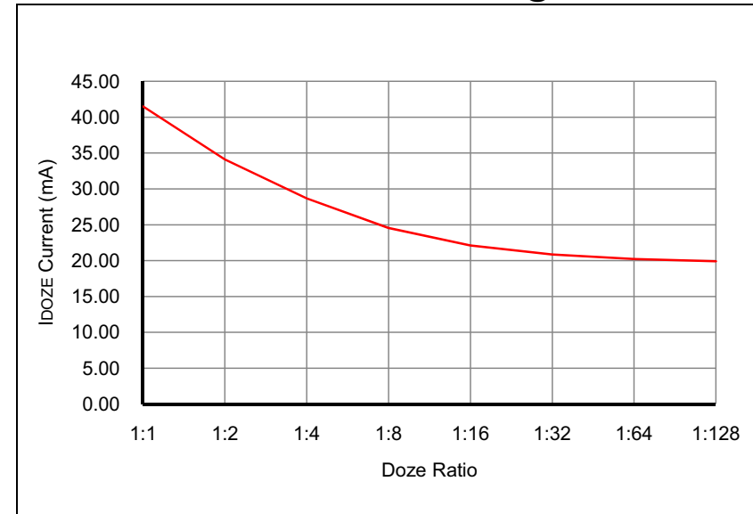
FIGURE 32-7: TYPICAL I DOZE CURRENT @ V DD = 3.3V
