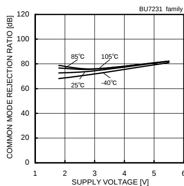
Fig. 62 Common Mode Rejection Ratio – Supply Voltage ( V_{DD}=3[V] )
