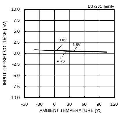
Fig. 58 Input Offset Voltage – Ambient Temperature ( V_{icm}=V_{DD} , V_{out}=0.1[V] )
