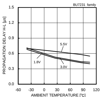
Fig. 66 Propagation Delay H-L – Ambient Temperature
