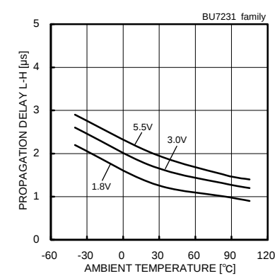
Fig. 65 Propagation Delay L-H – Ambient Temperature
