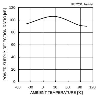
Fig. 64 Power Supply Rejection Ratio – Ambient Temperature
