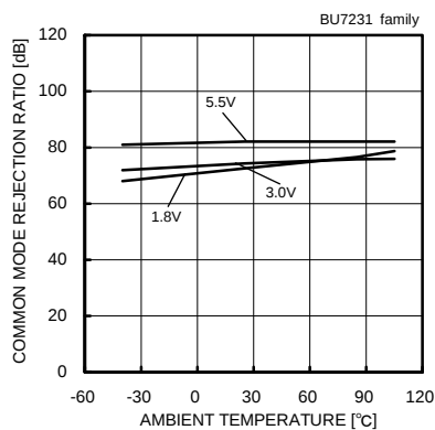
Fig. 63 Common Mode Rejection Ratio – Ambient Temperature ( V_{DD}=3[V] )
