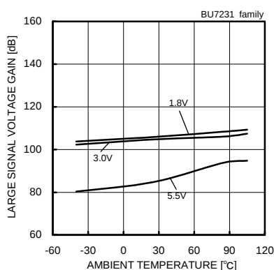
Fig. 61 Large Signal Voltage Gain – Ambient Temperature
