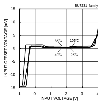
Fig. 59 Input Offset Voltage – Input Voltage ( V_{DD}=3[V] )
