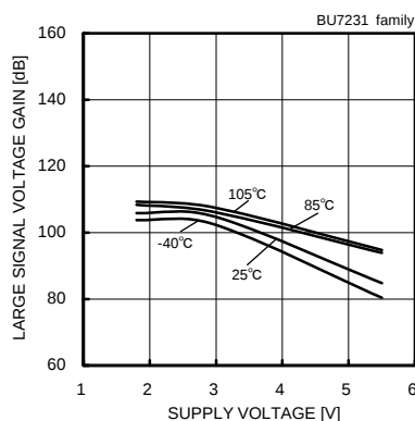
Fig. 60 Large Signal Voltage Gain – Supply Voltage
