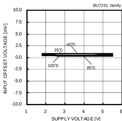
Fig. 57 Input Offset Voltage – Supply Voltage ( V_{icm}=V_{DD} , V_{out}=0.1[V] )
