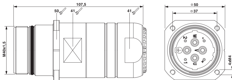
Dimensioned drawing
