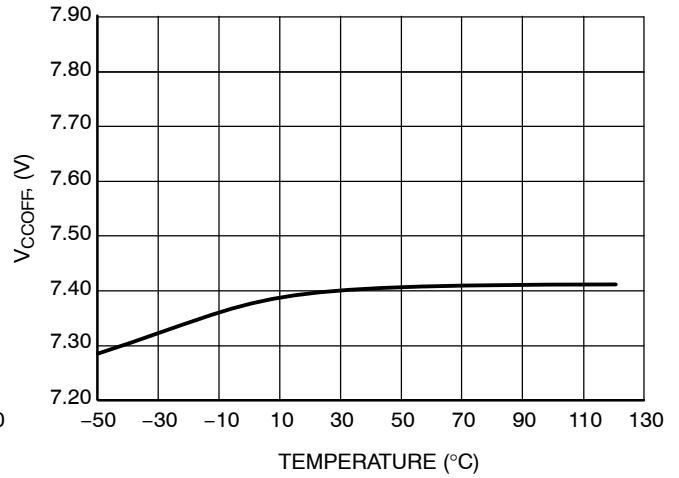
Figure 4. V COFF Threshold versus Temperature
