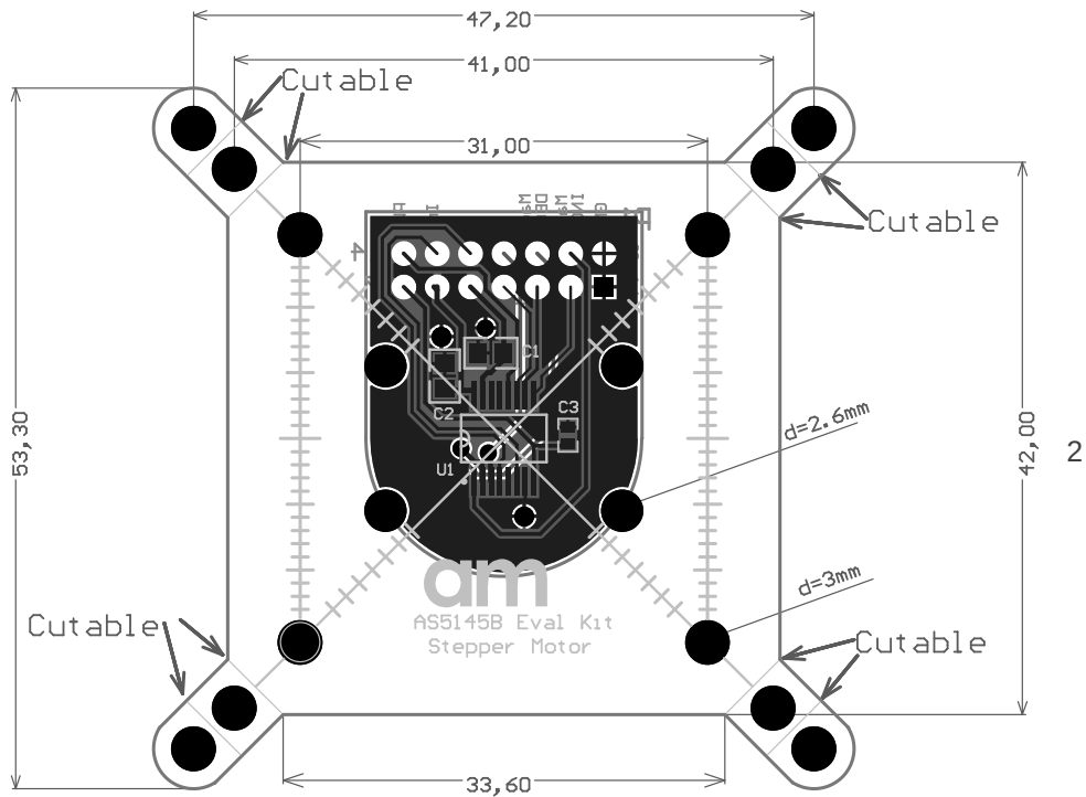
Figure 10: Layout Dimensions
