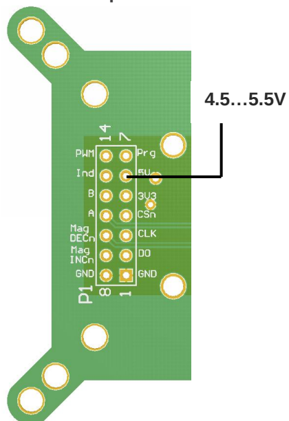
Figure 2: 5V Power Option
