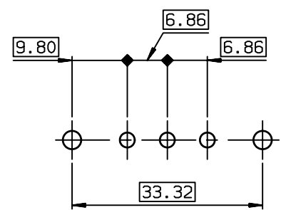
LAYOUT DIMENSIONS (after plating) CONNECTOR SIDE VIEW
