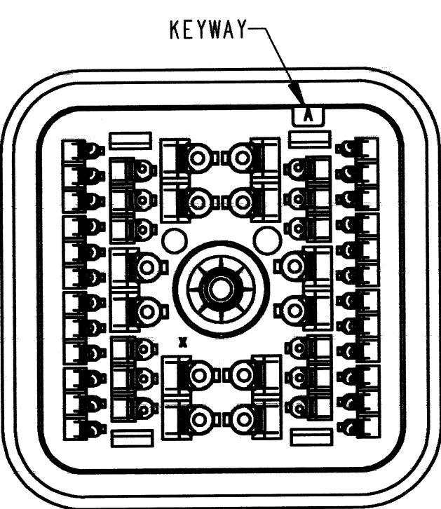
DRB16-48SAE-L018 KEY ARRANGEMENT -A-
