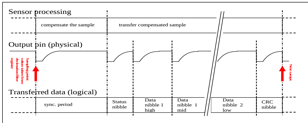
Figure 11 SENT Frame
