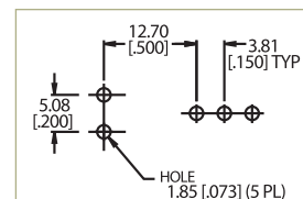
P.C. MOUNTING
