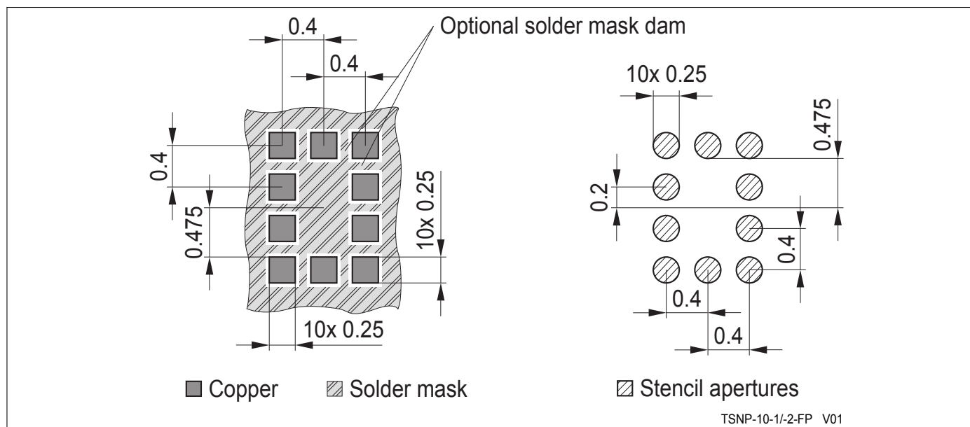
Figure 5: Land pattern and stencil mask (TSNP-10-1/-2)
