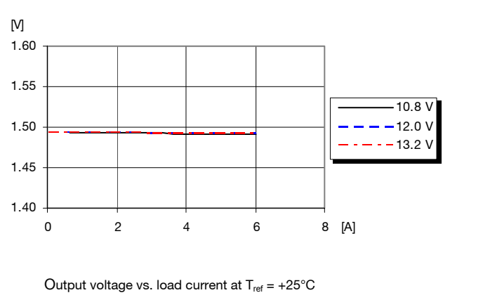
Output Characteristics
