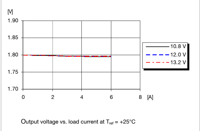
Output Characteristics
