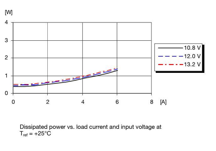
Power Dissipation
