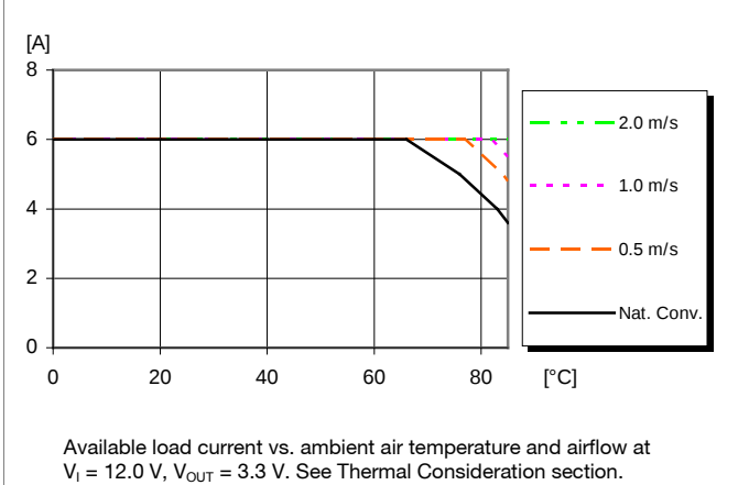
Output Current Derating
