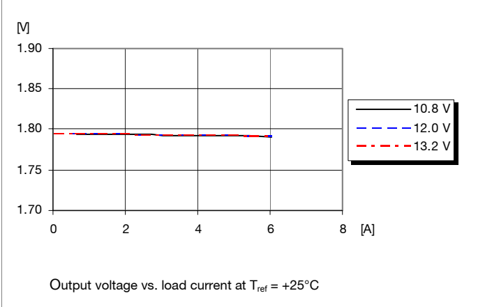
Output Characteristics
