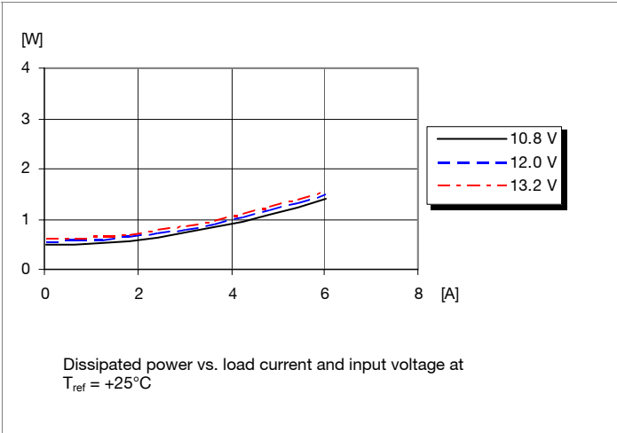
Power Dissipation
