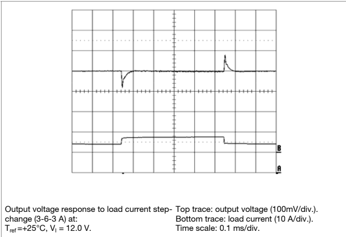
Output Load Transient Response
