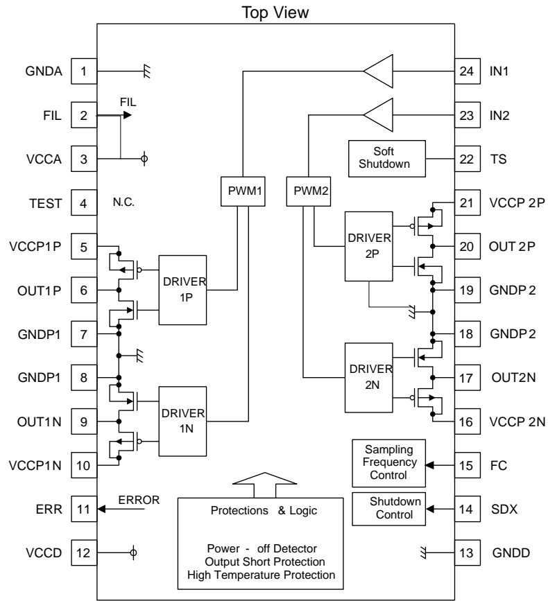
Fig. 26 Pin Assignment
