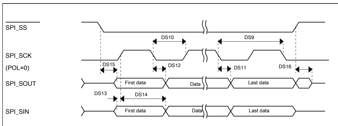
Figure 32. DSPI classic DSPI timing — slave mode
