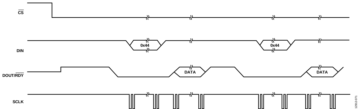
Figure 66. Continuous Conversion Mode
