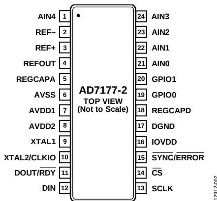
Figure 4. Pin Configuration
