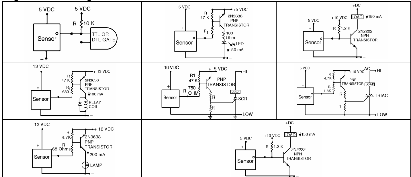
Figure 2. Interface Diagrams
