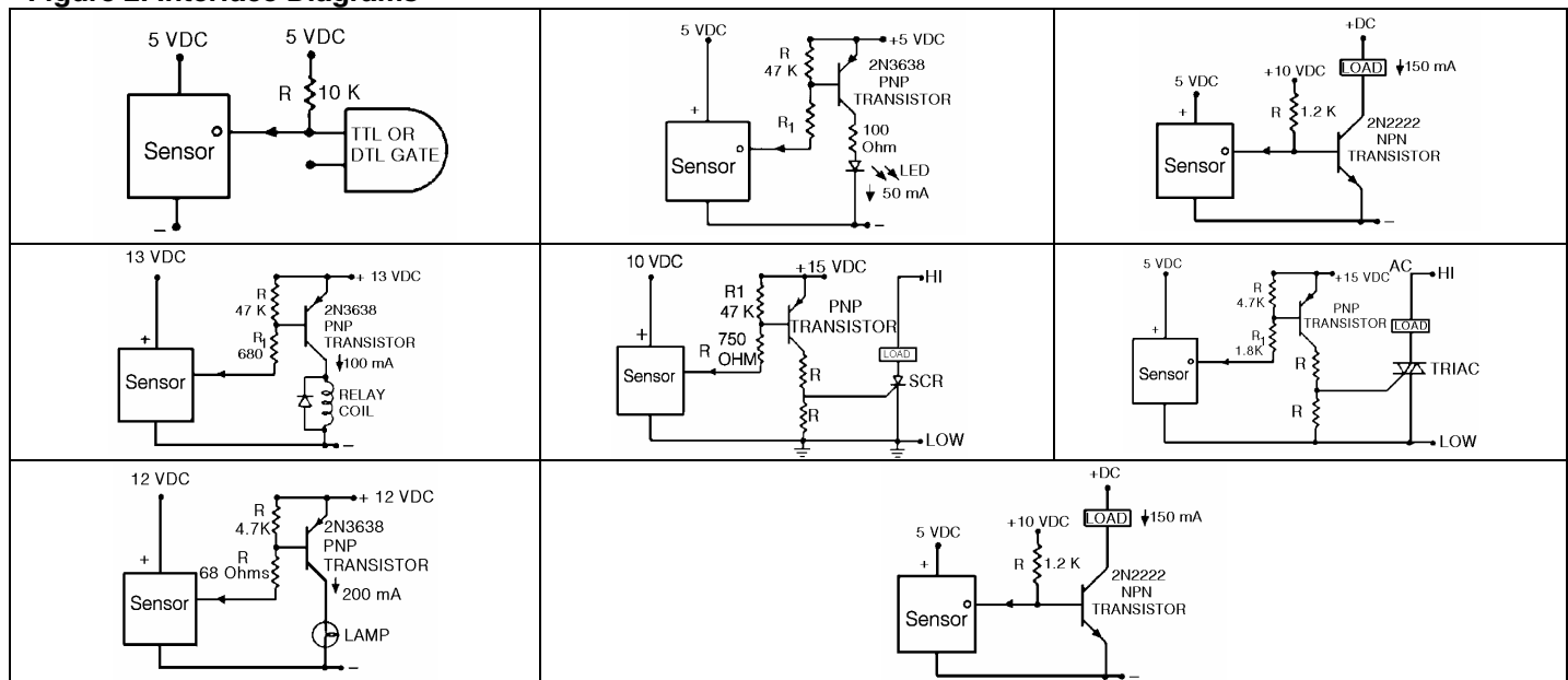
Figure 2. Interface Diagrams
