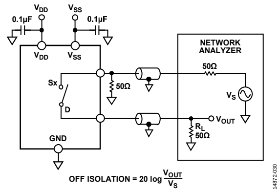
Figure 34. Off Isolation
