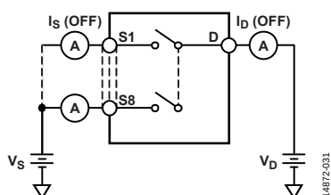
Figure 32. Off Leakage
