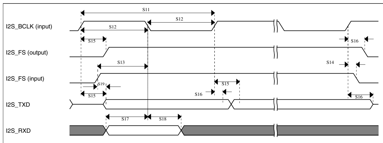
Figure 33. I²S timing — slave modes
