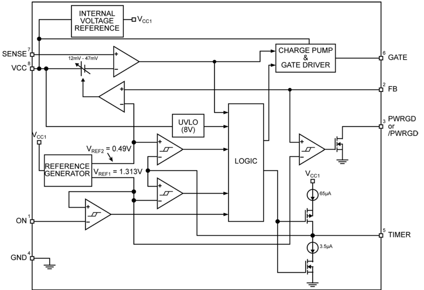
MIC2587/MIC2587R Block Diagram
