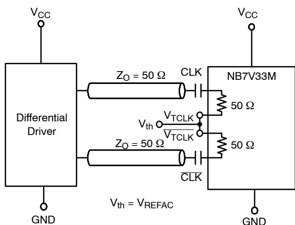
Figure 14. Capacitor-Coupled Differential Interface ( V_{TCLK}/V_{TCLK} Connected to V REFAC ; V REFAC Bypassed to Ground with 0.1 μF Capacitor)
