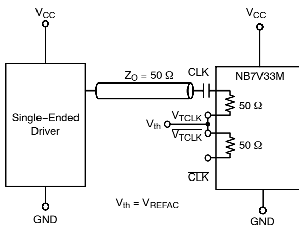
Figure 15. Capacitor-Coupled Single-Ended Interface ( V_{TCLK}/V_{TCLK} Connected to V REFAC ; V REFAC Bypassed to Ground with 0.1 μF Capacitor)
